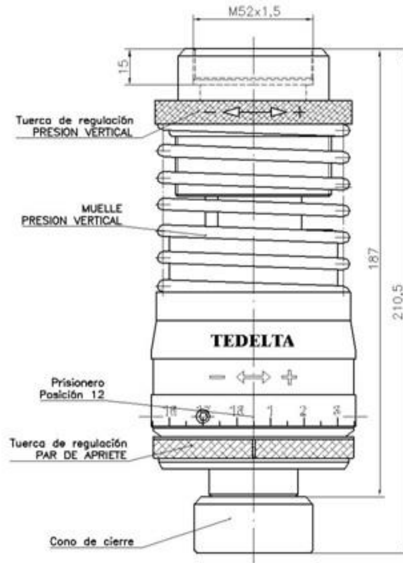
CABEZAL MAGNETICO TEDELTA-CM-706-TR VERSION "TRANSFER" (Pick and Place)
